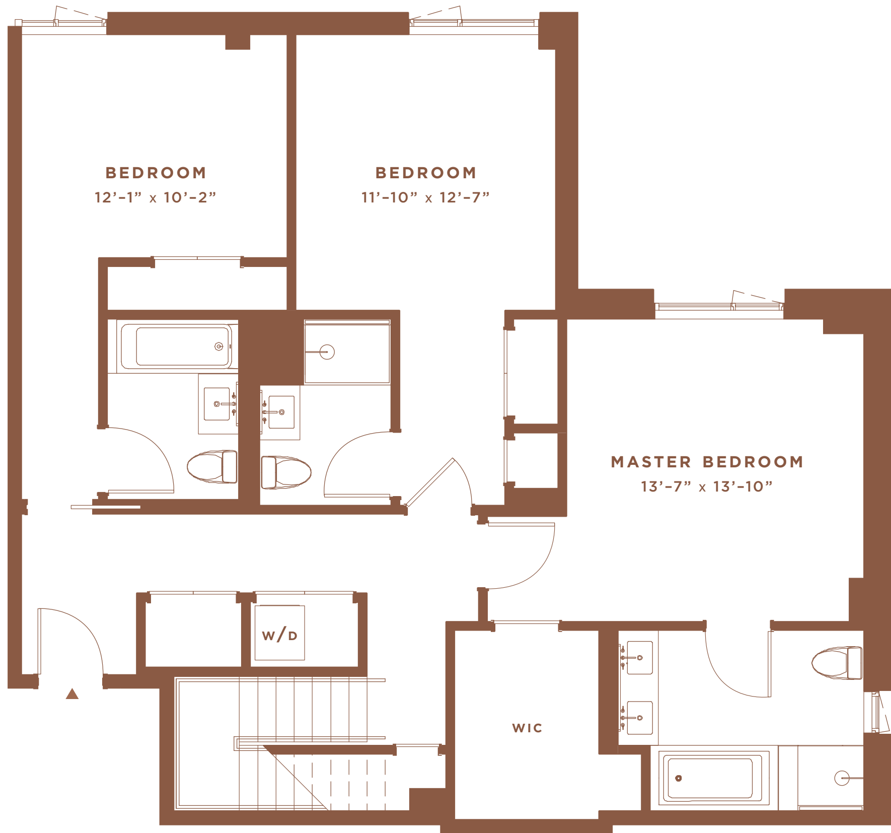
- FOURTH FLOOR -
